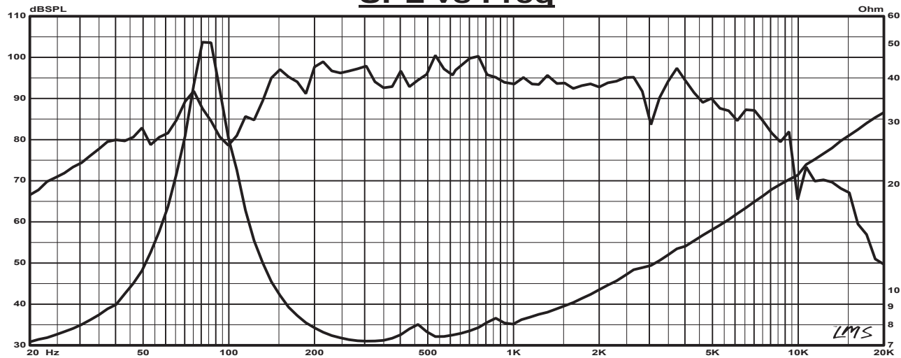
SPL vs Freq
